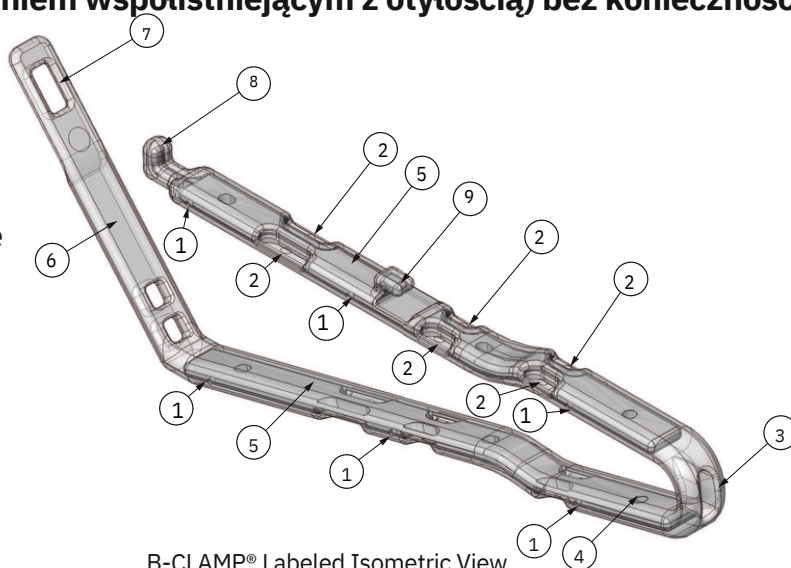
B-CLAMP® Labeled Isometric View
